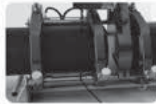
3. Place facing tool and start to cut surface of both pipes or fittings end .
